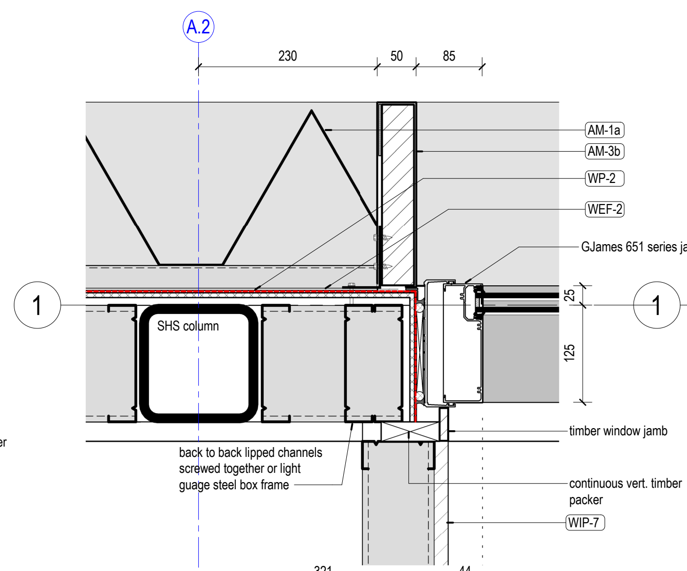
2 WEF-21 Window Jamb @ High Level 1:5
