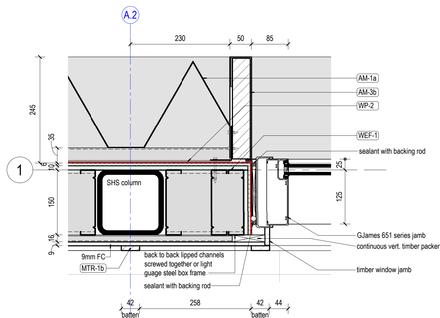
1 WEF-21 Window Jamb 1 : 5 Typical Window Jamb
