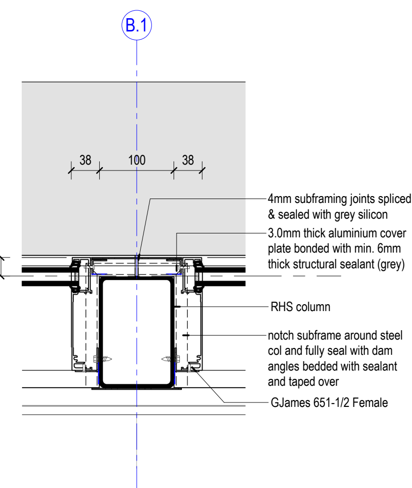
4 WEF-21 Window Column 1 : 5 Typical
